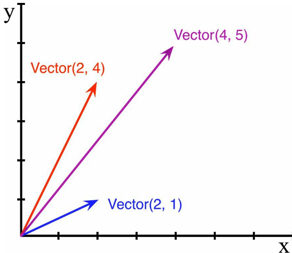
图 1-1: 一个二维向量加法的例子, \text{Vector}(2,4) + \text{Vector}(2,1) = \text{Vector}(4,5)
